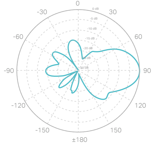
Horizontal Elevation
