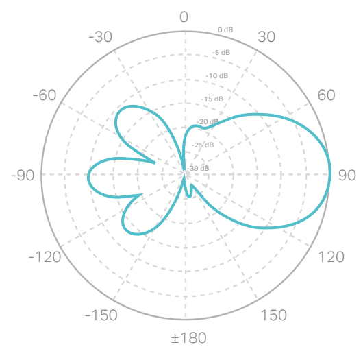
Horizontal Elevation
